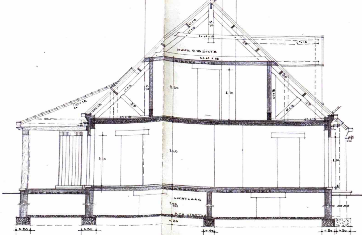
DOORSNED.
