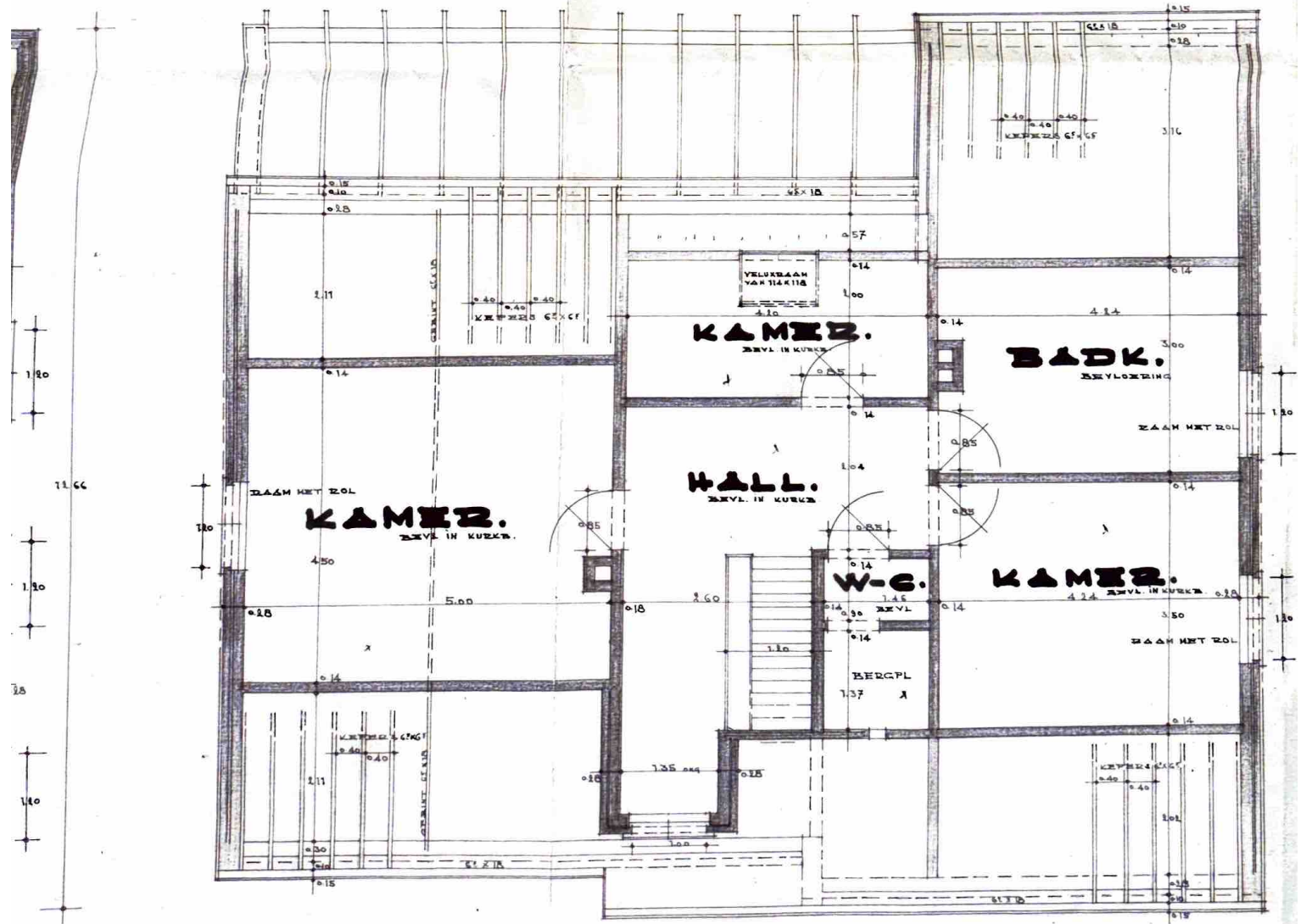
VERDIEPING.
