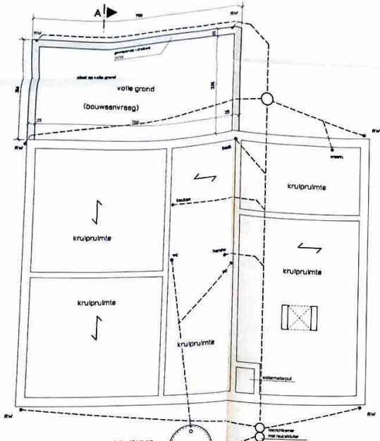
RIOLERING FUNDERING
