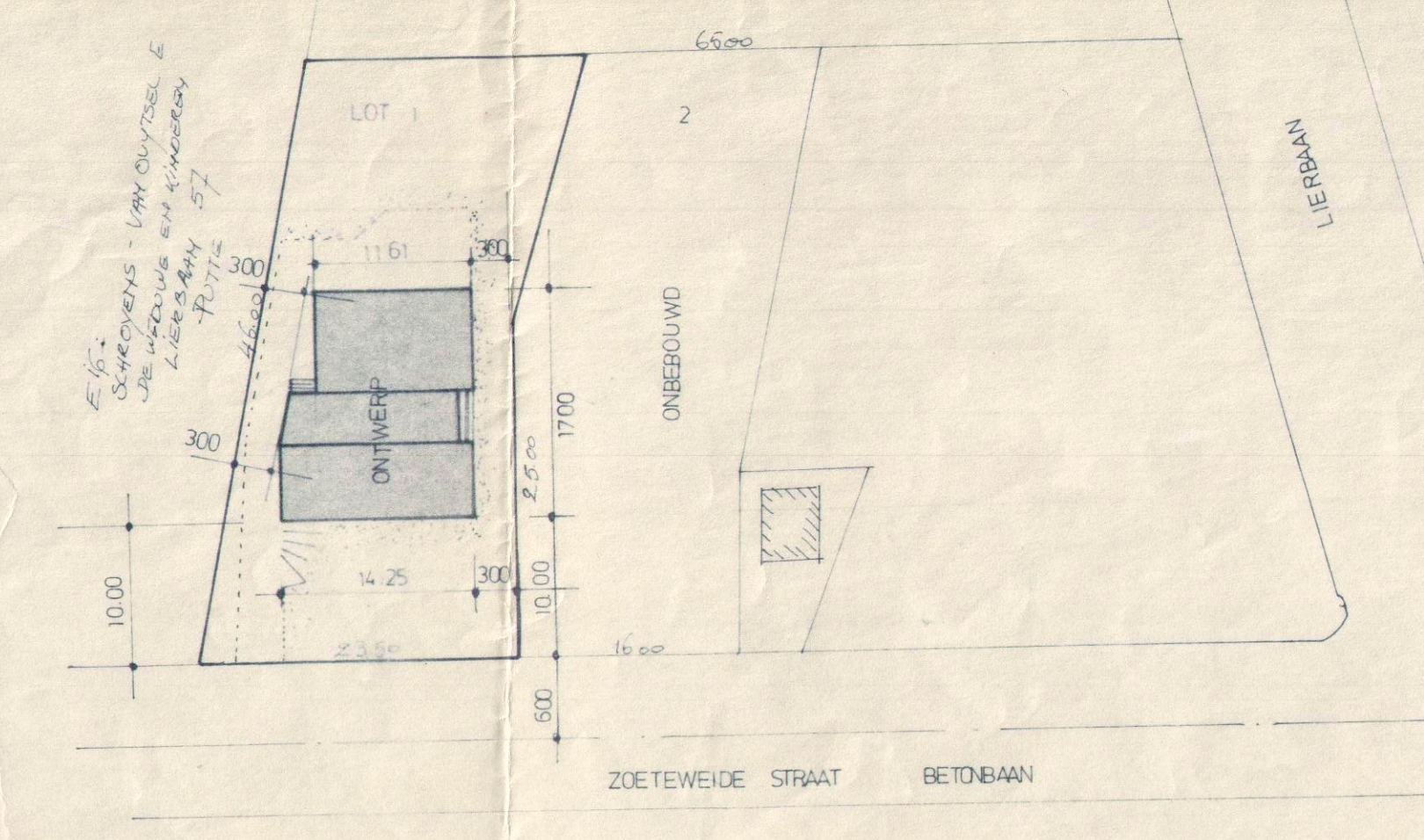
INPLANTINGSPLAN 1:500
