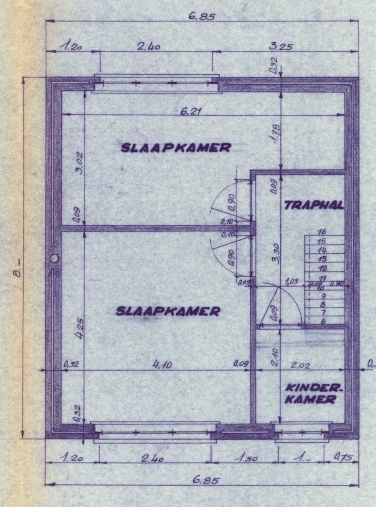
VERDIEPING.
